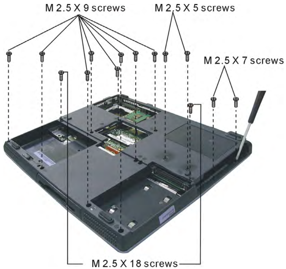
Figure 5-37: Removing 14 screws securing the top cover
