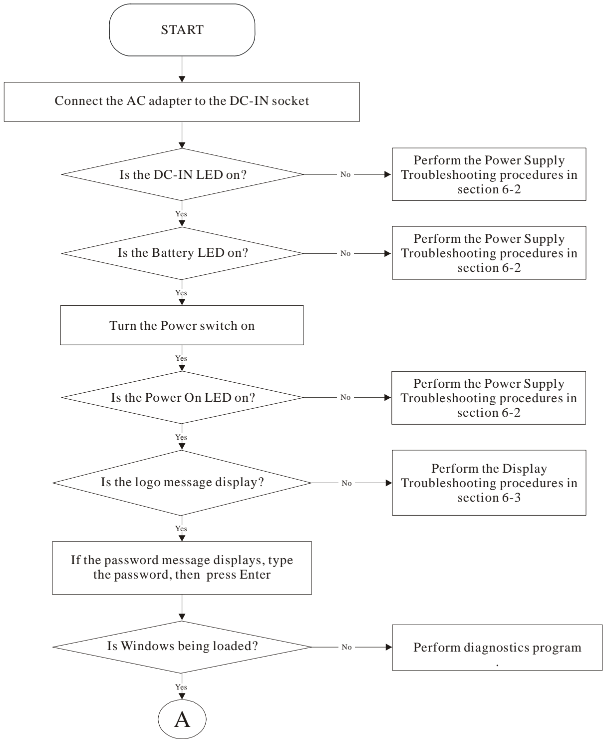
Figure 6-1 Troubleshooting flowchart (1/2)
