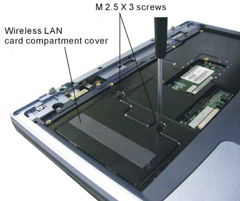
Figure 5-19: Removing the Wireless LAN compartment cover
