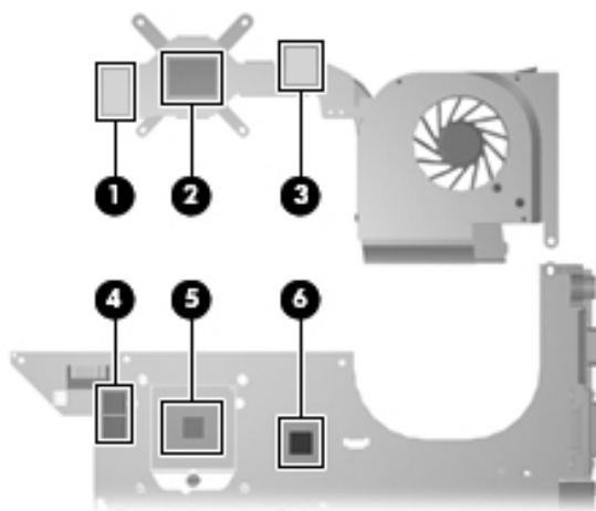
Thermal Pad and Thermal Paste Locations
