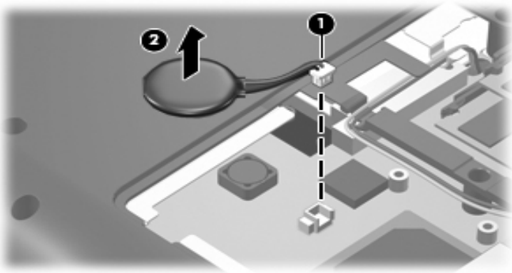
Removing the RTC Battery
