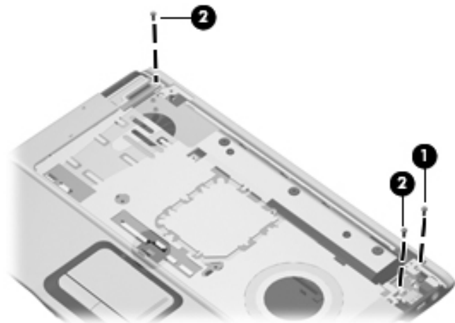
Removing the Top Cover Screws, Part 3
