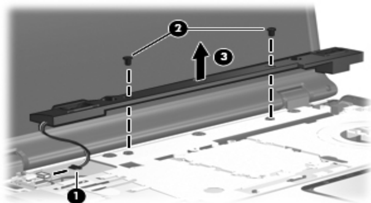
Removing the Speaker Assembly
