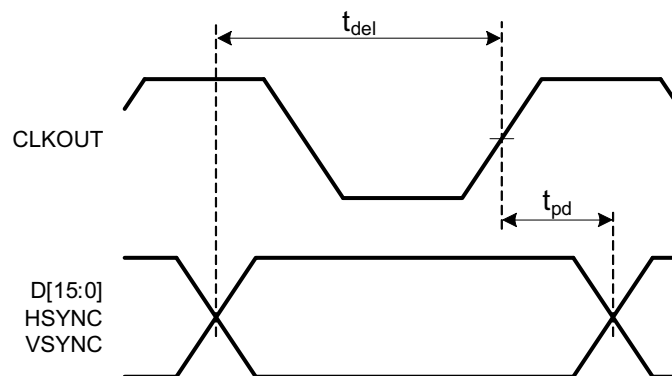
Figure 11. CMOS Output Timing Waveforms
