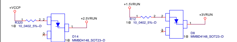
CRT DAC Voltage Follower Circuit - 700mV
