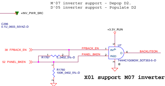
M'07 inverter support - Depop D2. D'05 inverter support - Populate D2
