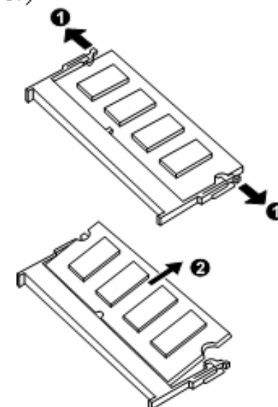
Figure 2-17 Remove the SO-DIMM
