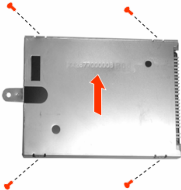
Figure 2-9 Remove hard disk drive
