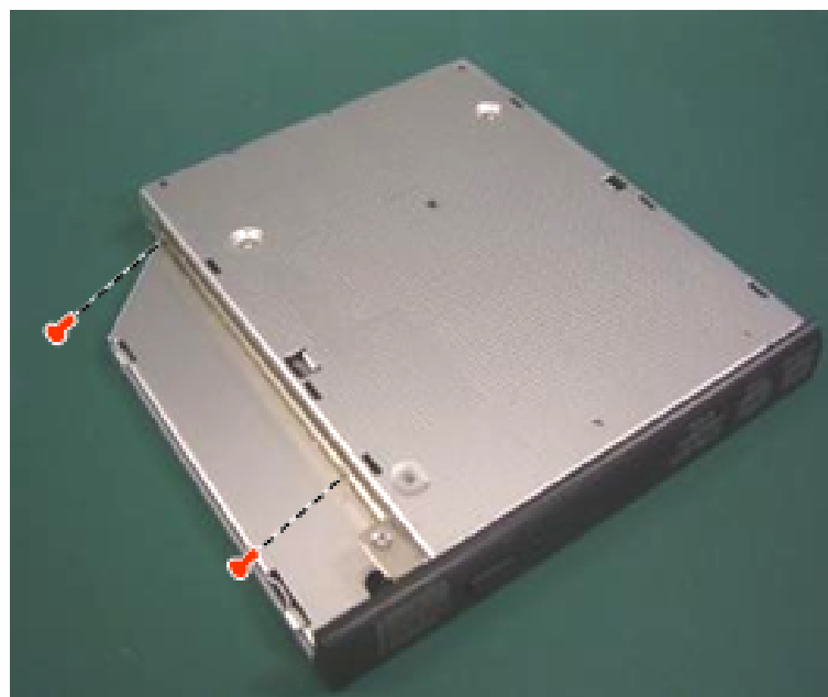
Figure 2-10 Remove 2 screw
