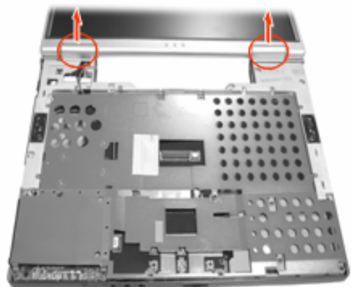
Figure 2-21 Remove the hinge covers
