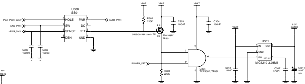
PDA POWER
