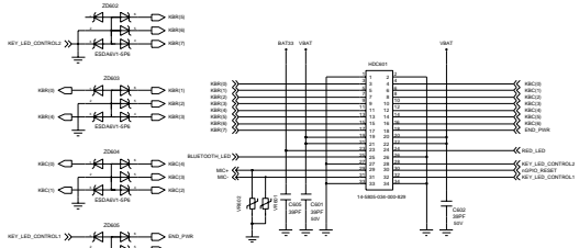
KEY CONNECTOR
