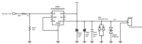
3.3V REGULATOR
