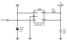
VCC_MEMORY
