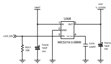
LCD_VOLTAGE
