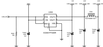
CAMERA VOLTAGE
