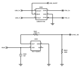
USB 1.1
