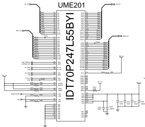
1.8V-1.8V DPRAM
