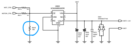
3.3V REGULATOR
