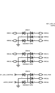
KEY CONNECTOR
