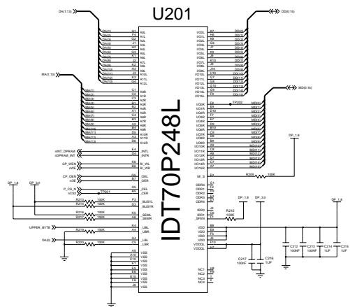
1.8V-3V DPRAM
