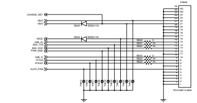
IF CON(Forward type)
