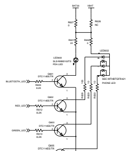
STATUS LED
