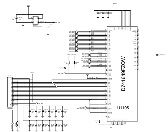
TIC (1.7)
