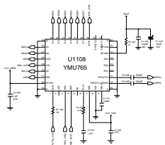
MELODY IC (64 POLY)
