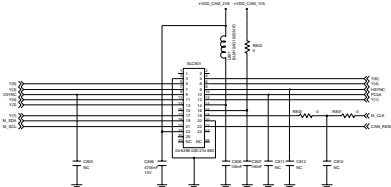
CAM_CONNECTOR
