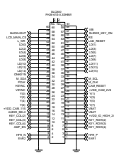
LCD_CONNECTOR
