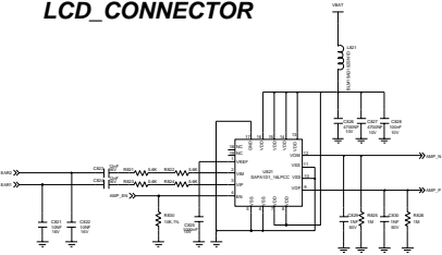
LCD_CONNECTOR
