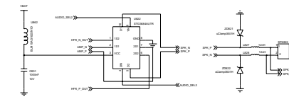
AUDIO
