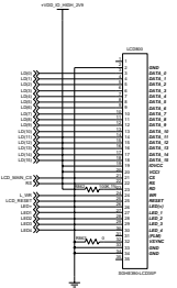
2" QCIF LCD
