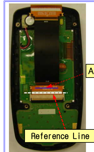
MAIN FPCB
