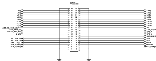
MAIN CONNECTOR
