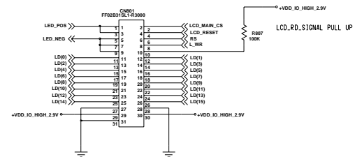
TFT LCD CONNECTOR
