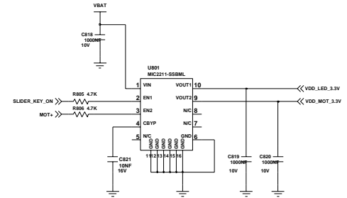
3.3 DUAL LDO
