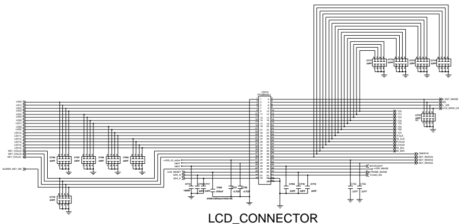
LCD_CONNECTOR
