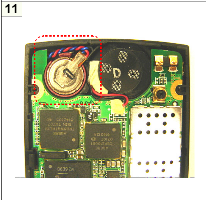
Assembly of MOTOR Assemble MOTOR into the external part
