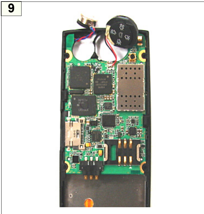
Assembly of PBA Insert PBA into the external part
