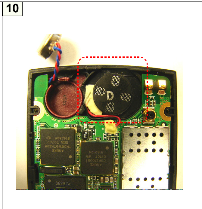
Assembly of SPEAKER Assemble SPEAKER into the external part
